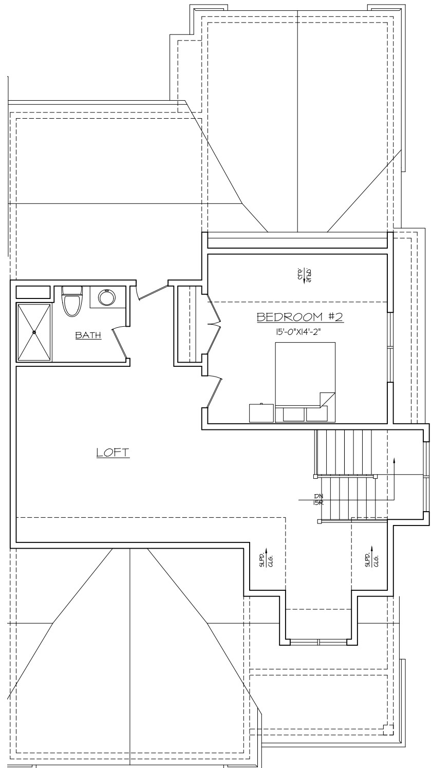
SECOND FLOOR | 862 SF
