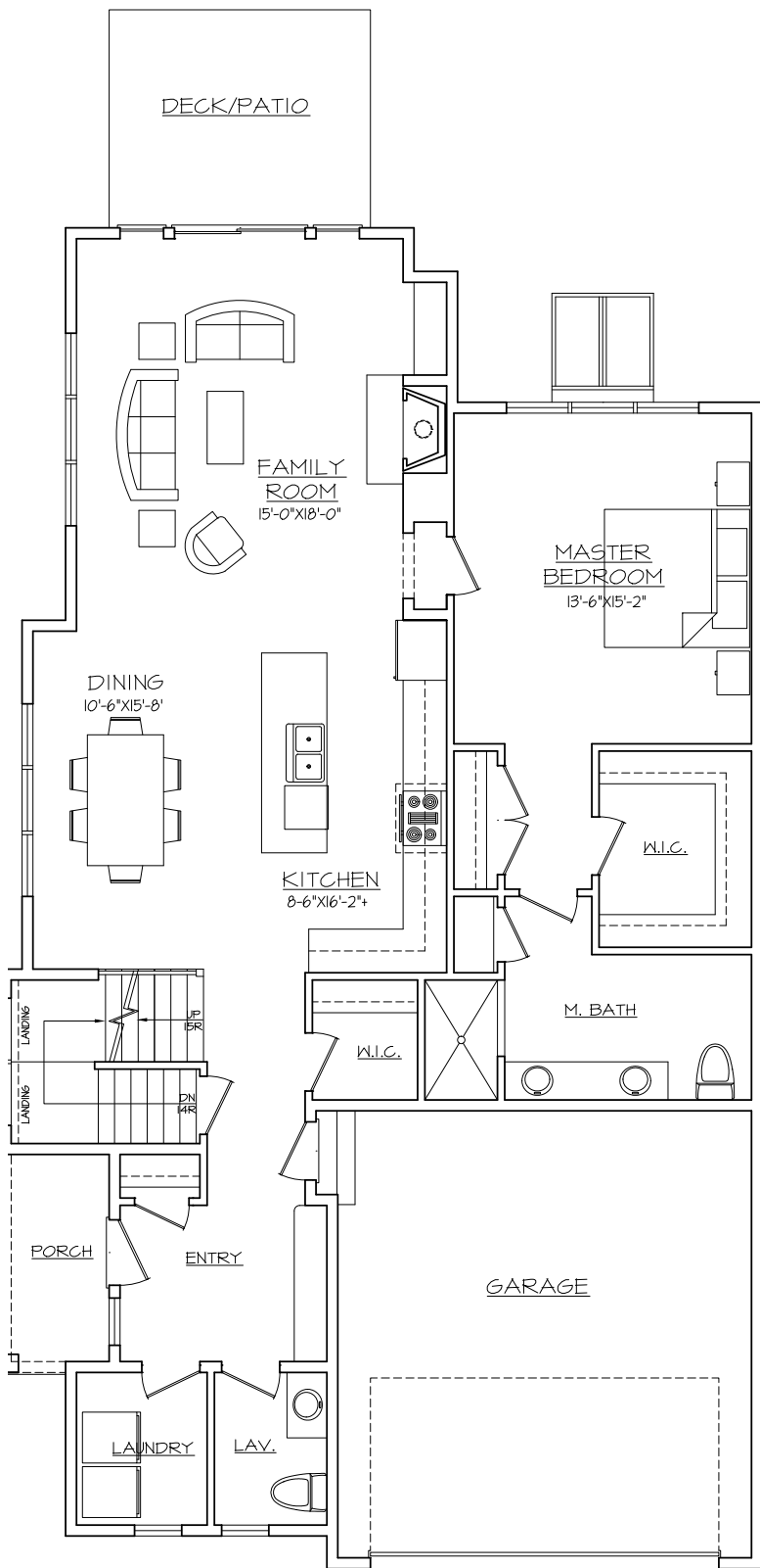
FIRST FLOOR | 1,458 SF
